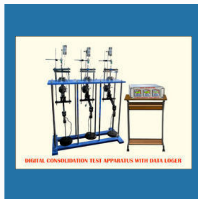
Digital Consolidation Test Apparatus with Data Logger
