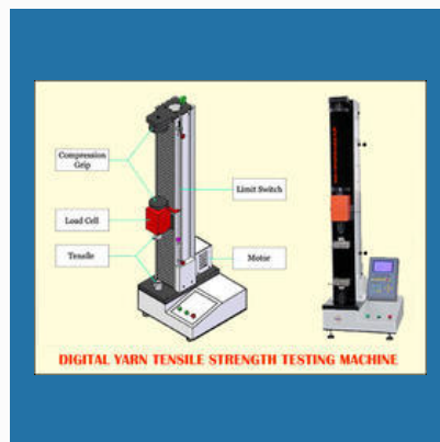
Fabrics Tensile Strength Testing Machine -50 KN
