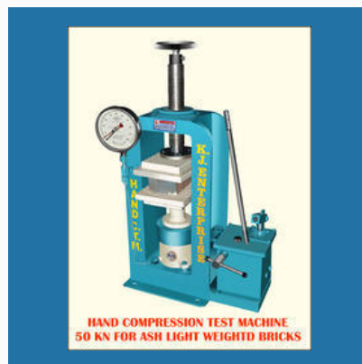
Hand Operated Concrete Testing Machine 500 Kn
